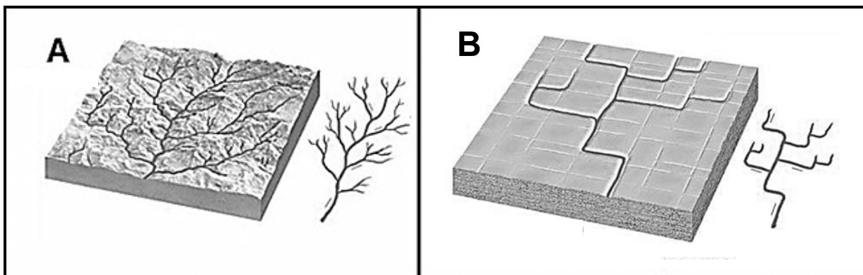
FIGURE 2.5: DRAINAGE PATTERNS
