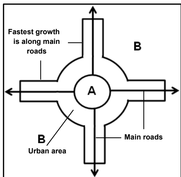
FIGURE 4.3: URBAN EXPANSION
