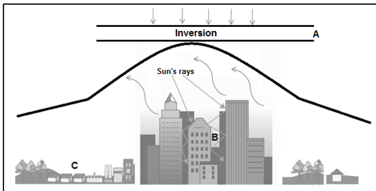
FIGURE 2.1: CITY CLIMATES
