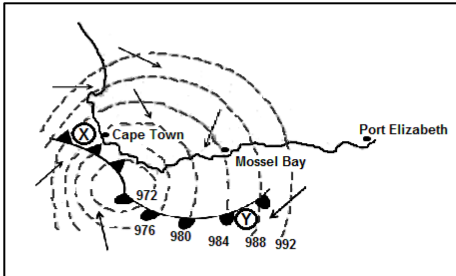
FIGURE 1.4: MID-LATITUDE CYCLONE
