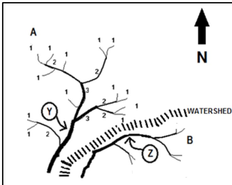
FIGURE 1.5: DRAINAGE BASINS
