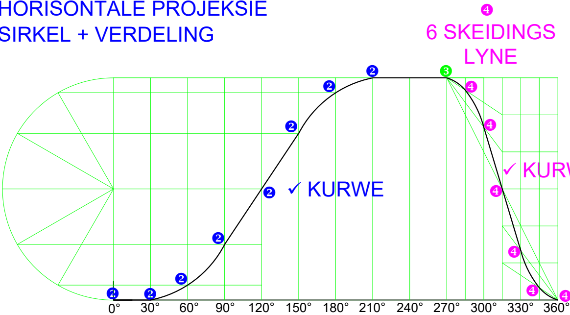
5 NOKVERPLASINGS DIAGRAM 5 SKAAL 360° = 120 MM
