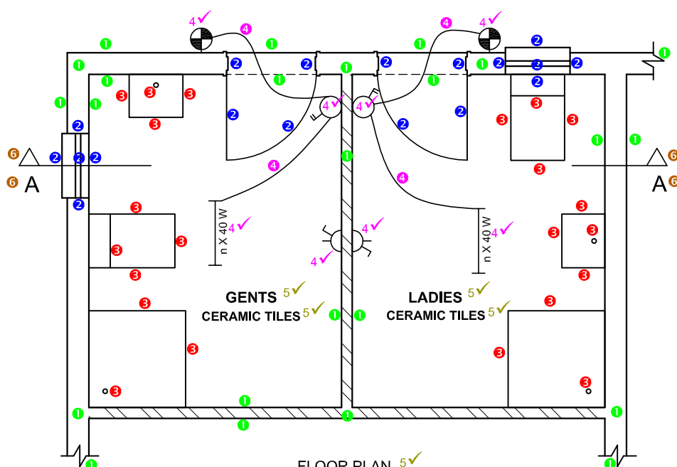
FLOOR PLAN 5✓ SCALE 1 : 50 5✓
