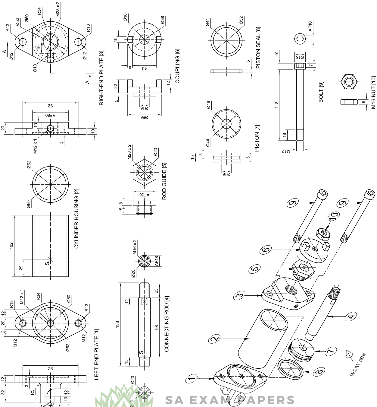
EXPLODED ISOMETRIC DRAWING
