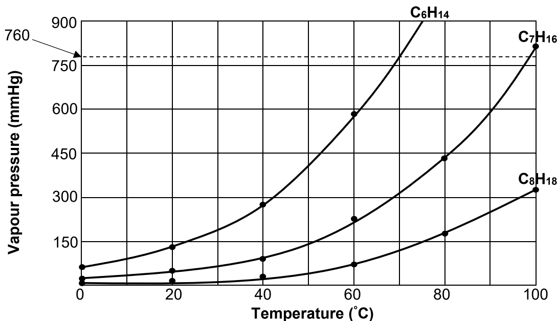
GRAPH OF VAPOUR PRESSURE VERSUS TEMPERATURE
